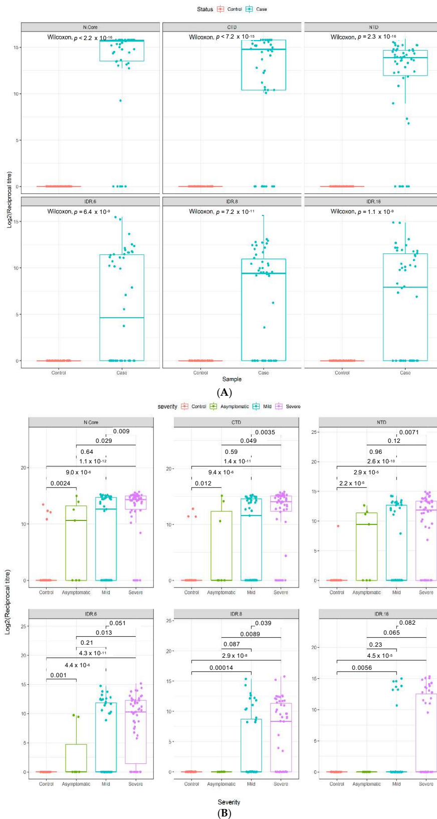
Figure 1. Epitope selectivity of IgG responses in two independent COVID-19 cohorts. Antibody reciprocal titers against different epitopes ( n = 6 ) of the SARS-CoV-2 N protein in two separate COVID-19 case and control cohorts. (A) Validation cohort ( n = 100 ), consisting of 50 hospitalized COVID-19 patients and 50 pre-pandemic controls (Cohort 2). (B) Multi-ethnic cohort ( n = 138 ), consisting of 50 severe COVID-19 patients, 50 mild COVID-19 patients, and 38 healthy controls (Cohort 3). Boxes represent the 25th and 75th percentiles, and the midline represents the median and whiskers represent the 5th and 95th percentiles. p -values were determined using the Wilcoxon test (unpaired, two-tailed).
